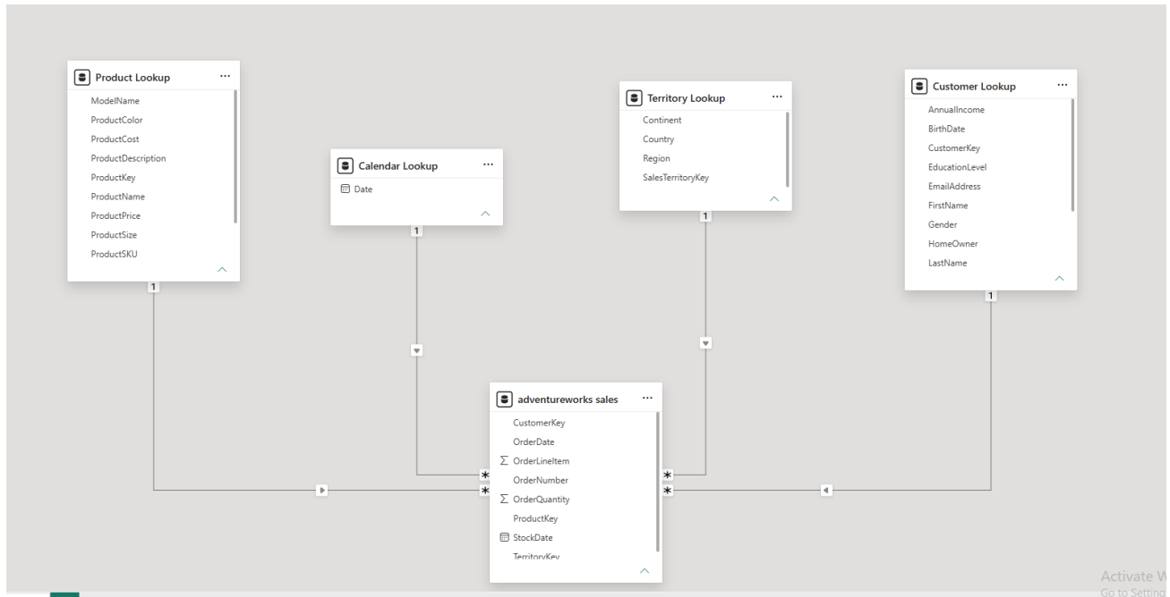
Figure 8: Data Model — Star Schema in Model View
